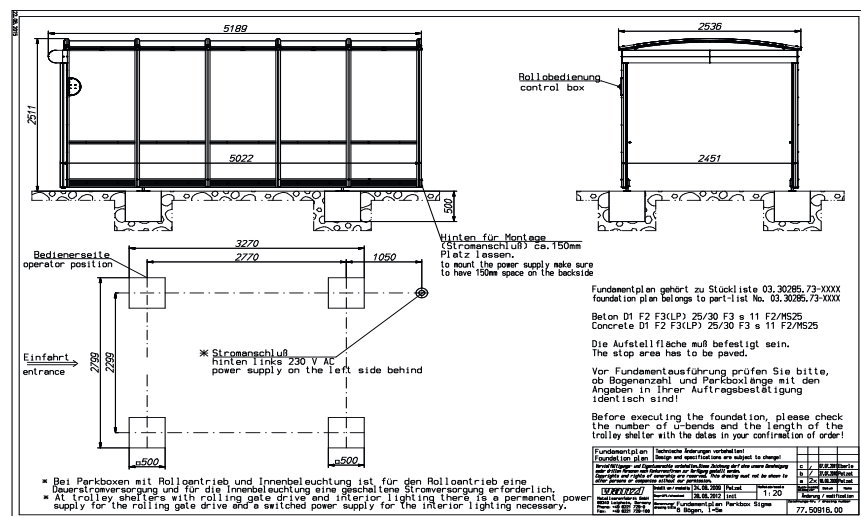
Sample foundation plan
