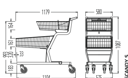
CUSTOMISED SHOPPING TROLLEY FOR WHEELCHAIR USERS 90
