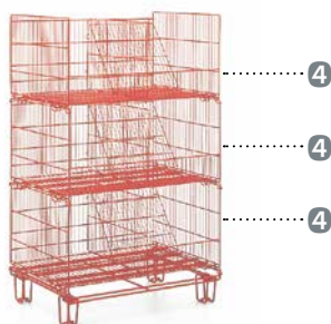
STP/R 810 colour coating (on request), with stationary chassis, dividers, sloping grates
