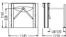
Sirio a 2 bracci "Open-gate"
