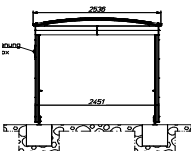
05 FOUNDATIONS FOR TROLLEY SHELTERS
