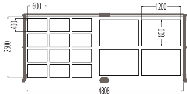
Sample plan of practical option for filling with pallets (bird's eye view)
