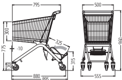
02 SHOPPING TROLLEY DIMENSIONS
