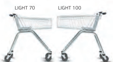
Basket volume of 70 or 100 litres.
