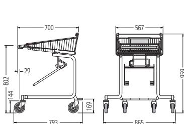
CUSTOMISED SHOPPING TROLLEY FOR WHEELCHAIR USERS 40
