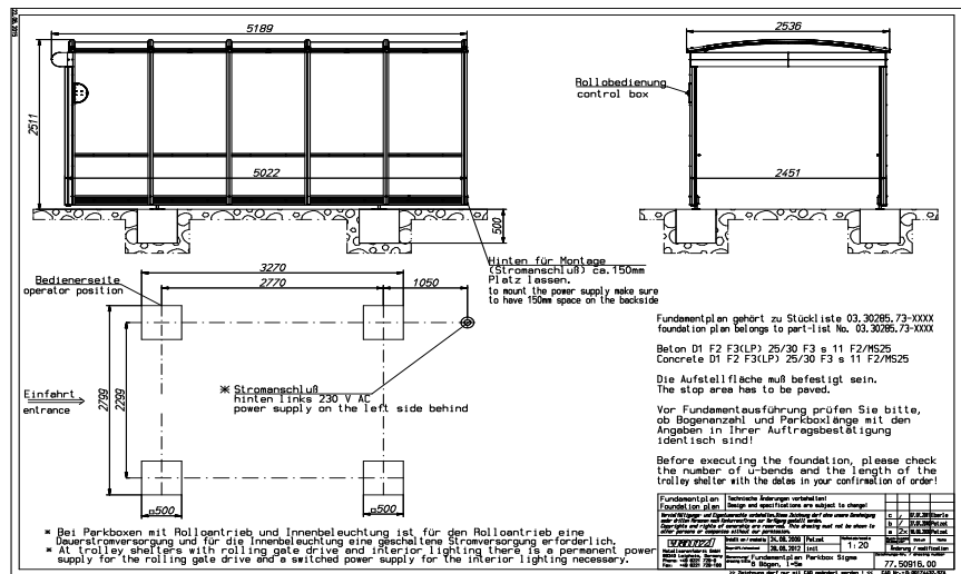
Sample foundation plan
