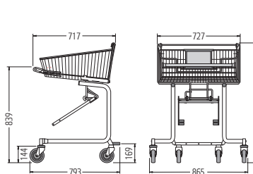
CUSTOMISED SHOPPING TROLLEY FOR WHEELCHAIR USERS 90
