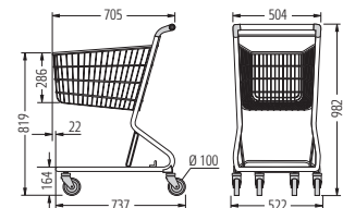
CS 60
