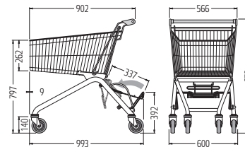
EL/ELX 101
