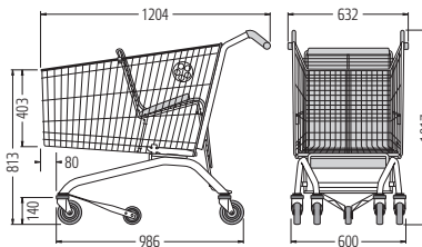
BEN'S CART
