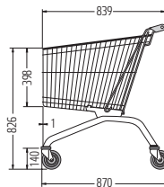
EL/ELX 101
