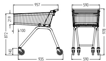
LIGHT 100
