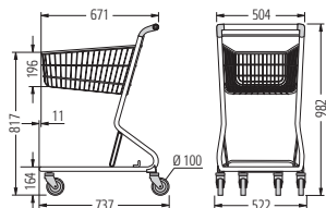
CS 40
