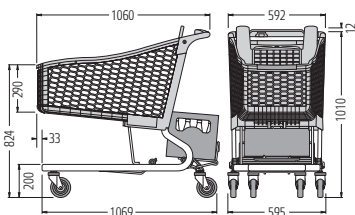
TANGO 160 P
