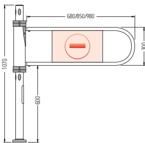
with Colour Classic swivel barrier
