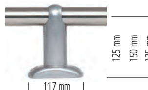
Rectangular foot , standard heights
