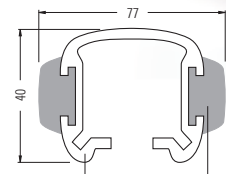
Aluminium profile Plastic bumper profile
