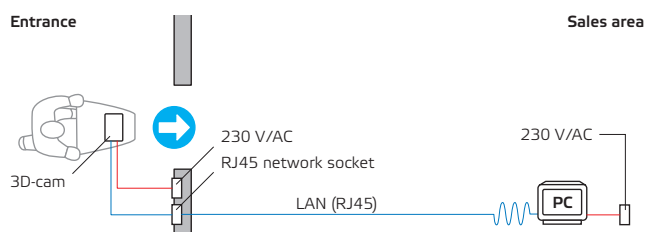
CUSTOMER COUNTER diagram with one counting point
