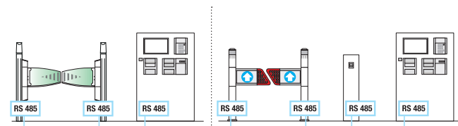
The ExitGates are connected and controlled via a LAN connection or the RS 485 stand- ard computer interface
