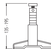
Foot, height-adjustable
