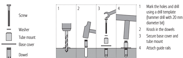
Installation for normal floor constructions, fixing materials supplied as standard
