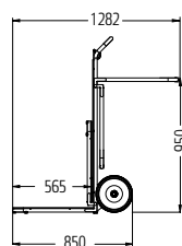
GS-Compact 600 A
