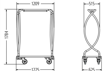
GS-TREND Electro-polished stainless steel Illustration shows optional equipment.
