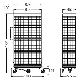
SHELVED LAUNDRY TROLLEY KT3 Illustration shows optional equipment
