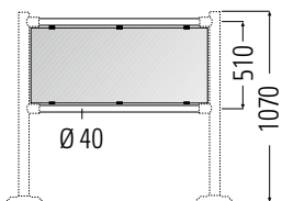
Partition element Suitable for uprights with 2 tubes
